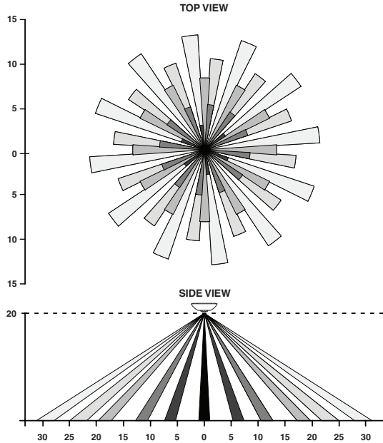
Figure 8 - (Mid-Range Lens) Field-of-View Ranges Mid range lens (red frame), mounting height (13-20 ft)
