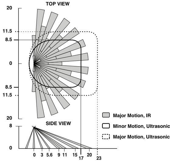
Figure 7 (Cat. No. ODC10) Field-of-View Ranges
