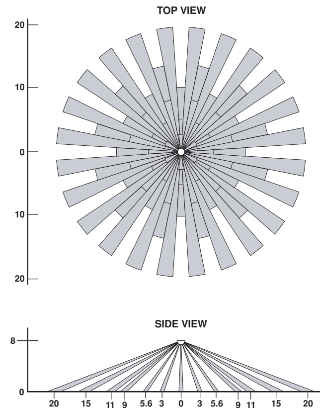
Figure 3 (Cat. No. OSC15) Field-of-View Ranges
